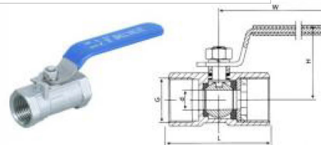
1PC不锈钢内螺纹球阀
