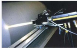
Supersonic Flame Spraying
