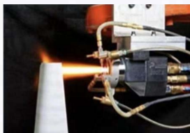
Plasma Spraying
